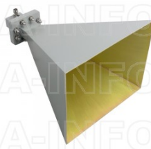
LB-159-20-C-TF Standard Gain Horn Antenna 4.9-7.05GHz 20dB Gain TNC Female
