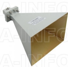
LB-159-20-C-SF Standard Gain Horn Antenna 4.9-7.05GHz 20dB Gain SMA Female
